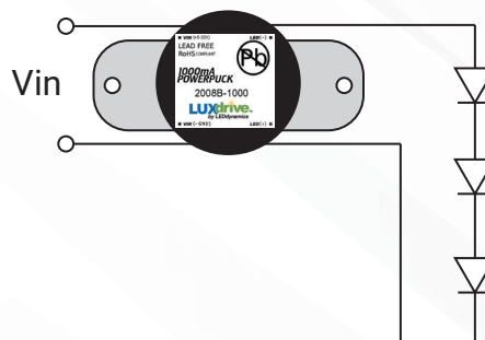
Figure 6. 1000mA unit driving three Luxeon® III emitters (VIN > 12VDC)
