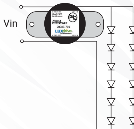
Figure 4. 700mA unit driving LumiLEDs 12-ring (VIN > 24VDC, IOUT limited to 600mA )
