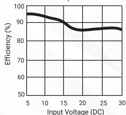
Figure 1. Efficiency vs. Vin
