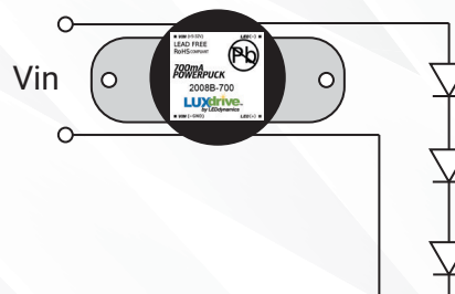
Figure 8. 700mA unit driving three Luxeon® V emitters (VIN > 24VDC)
