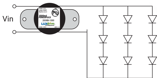
Figure 5. 1000mA unit driving nine Luxeon® I emitters (VIN > 12VDC)
