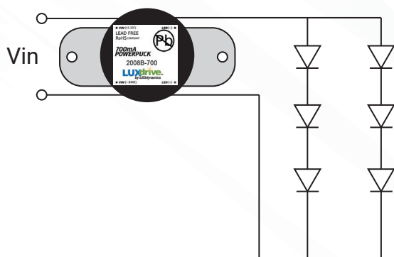
Figure 3. 700mA unit driving LumiLEDs 6-ring (VIN > 12VDC)
