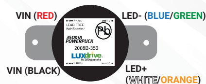
Figure 2. Wire Configuration
